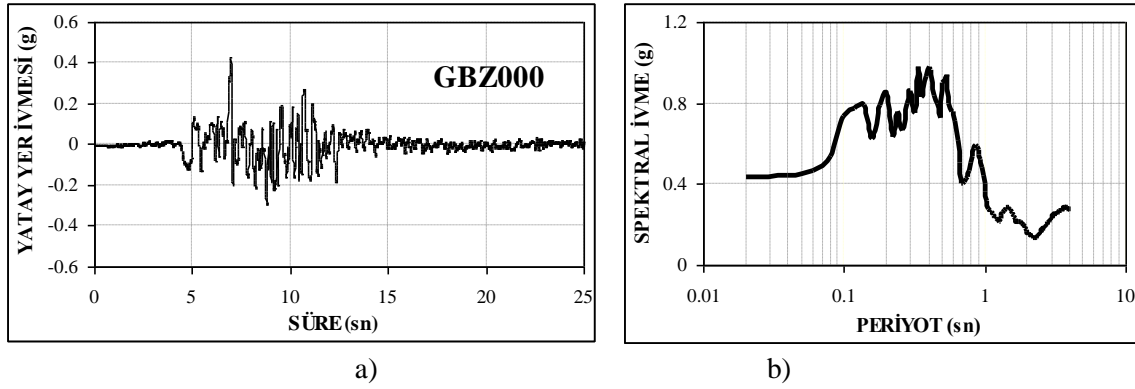
Figure 1. NS component of 1999 Kocaeli Earthquake, a) acceleration time-history scaled to PGA of 0.42g b) scaled acceleration spectra
